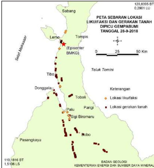
Figure 3.25. Map of the liquefaction distribution and landslide locations triggered by the earthquake on September 28 th , 2018 (Supartoyo et al. , 2018).
