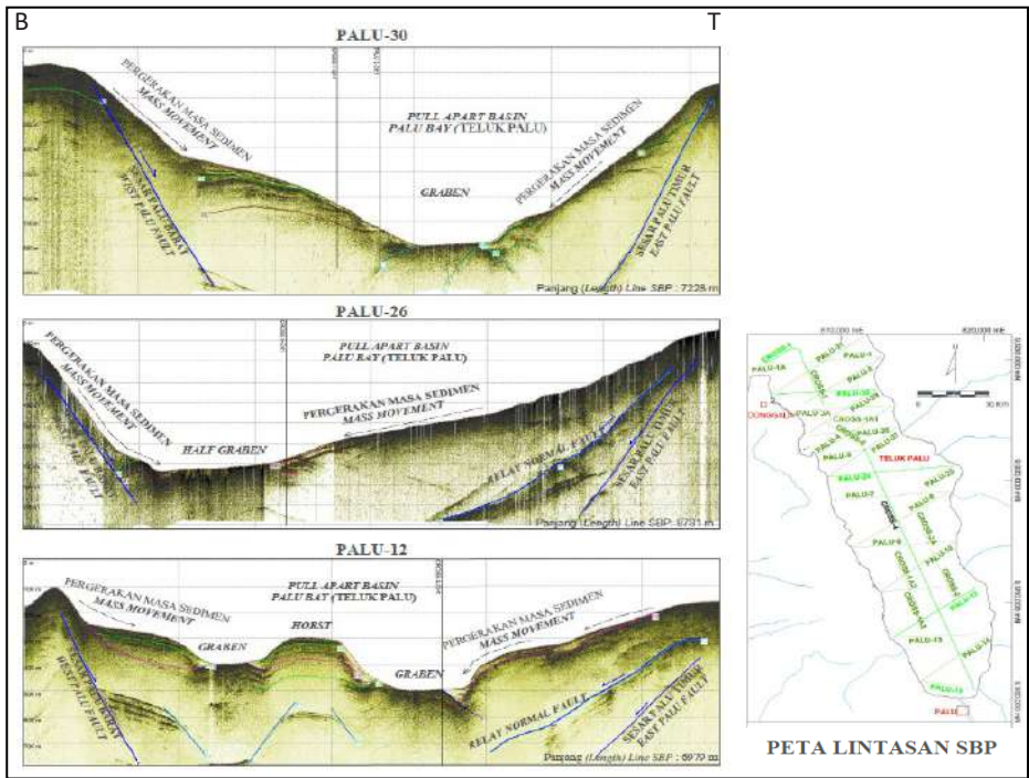
Figure 3.27. Shallow seismic line indicate submarine landslide area, as one of the tsunami triggers (Gustiantini et al. , 2024).
