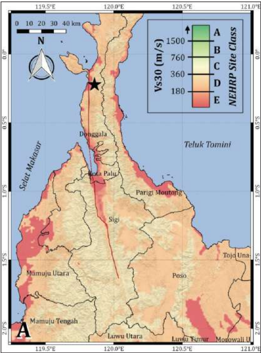
Figure 3.18. Map of shear wave velocity of thickness 30 m depth ( V_{s30} ) in Central Sulawesi Province and surrounding area. The red line is The Palu-Koro Fault that is used in deterministic hazard modeling, and the black star is an epicentre (Omang et al. , 2018).
