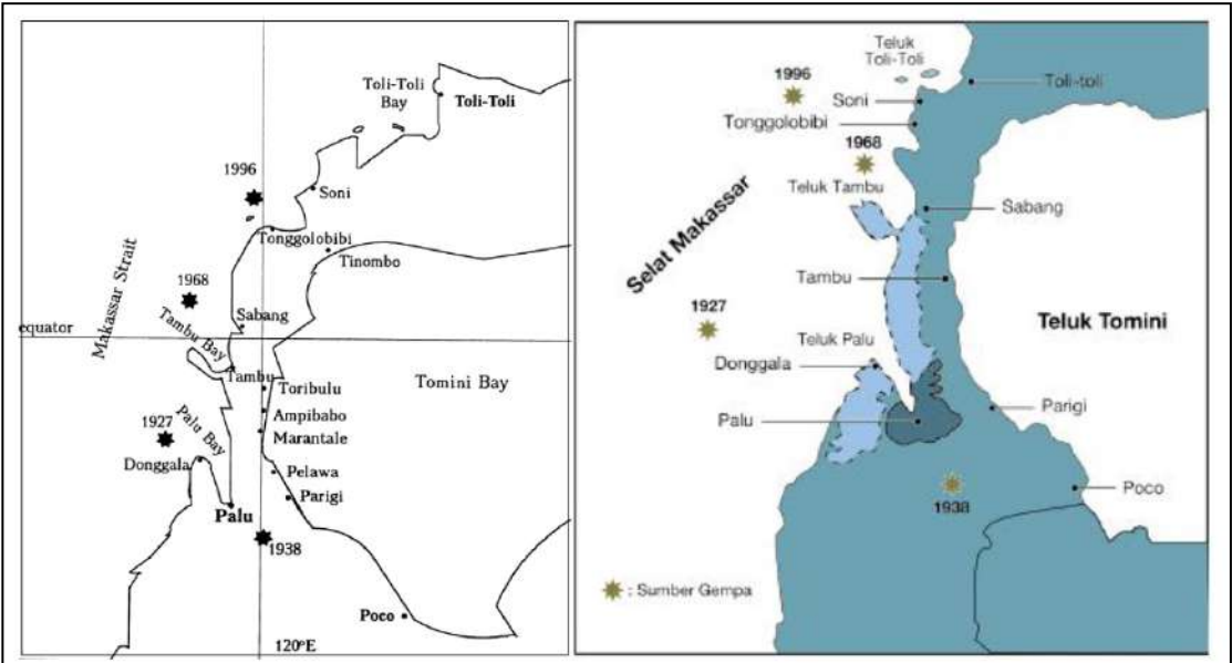
Figure 3.28. The earthquake epicentre resulting tsunami during one century occurred in the westcoast of Sulawesi (left); The earthquake centre triggered tsunamis surround Palu Bay prior to 2018 tsunami (right) (Pelynovsky et al. , 1997).
