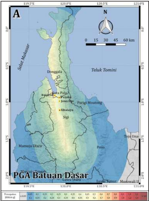
Figure 3.19. The earthquake shaking on bedrock (Omang et al. , 2018).
