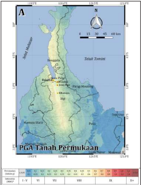
Figure 3.20. The earthquake shaking on surface (Omang et al. , 2018).
