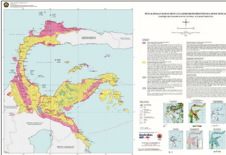
Figure 3.16. Map of earthquake-prone areas in Central Sulawesi (Robiana et al. , 2012).
