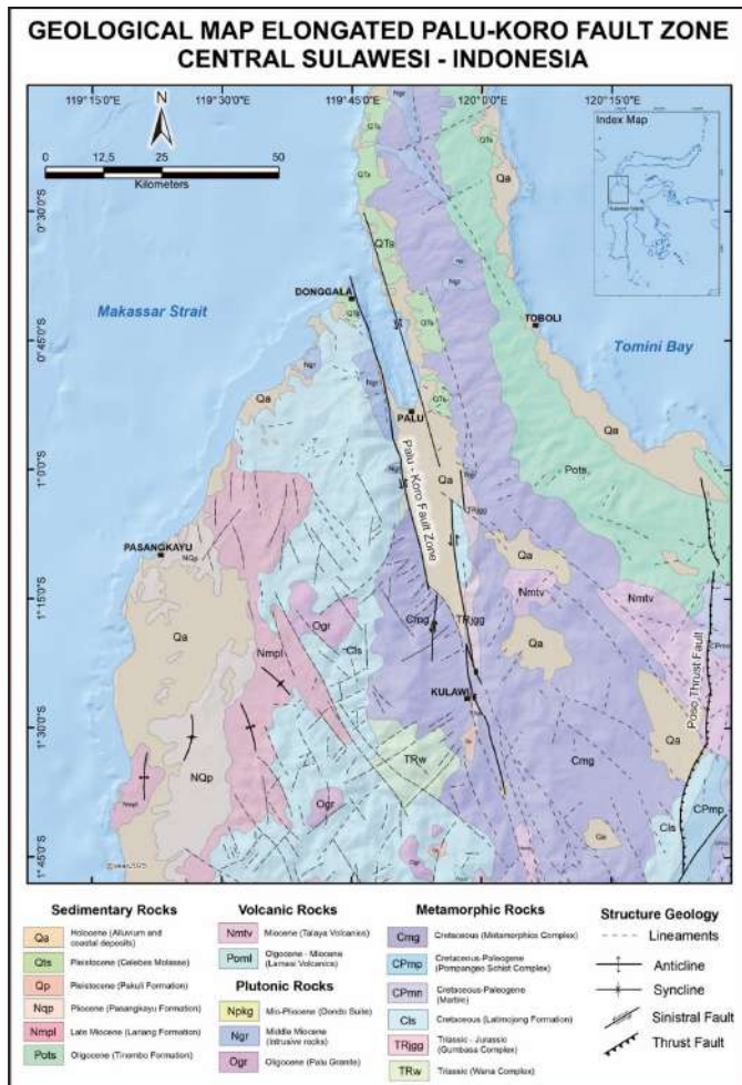
Figure 2.7. Geological map of the elongated Palu-Koro Fault, Central Sulawesi. The information has been adapted from the works of Sukanto in 1973, Simandjuntak et al. in 1997, and Sukido et al. in 2011.
