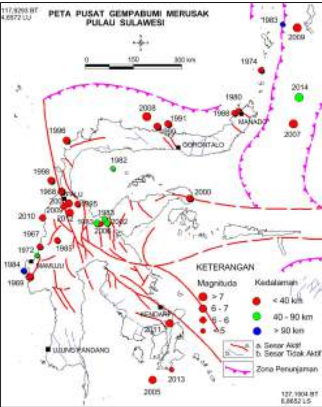
Figure 3.3. Map epicentre of destructive earthquake in Sulawesi Island (Supartoyo et al. , 2014).
