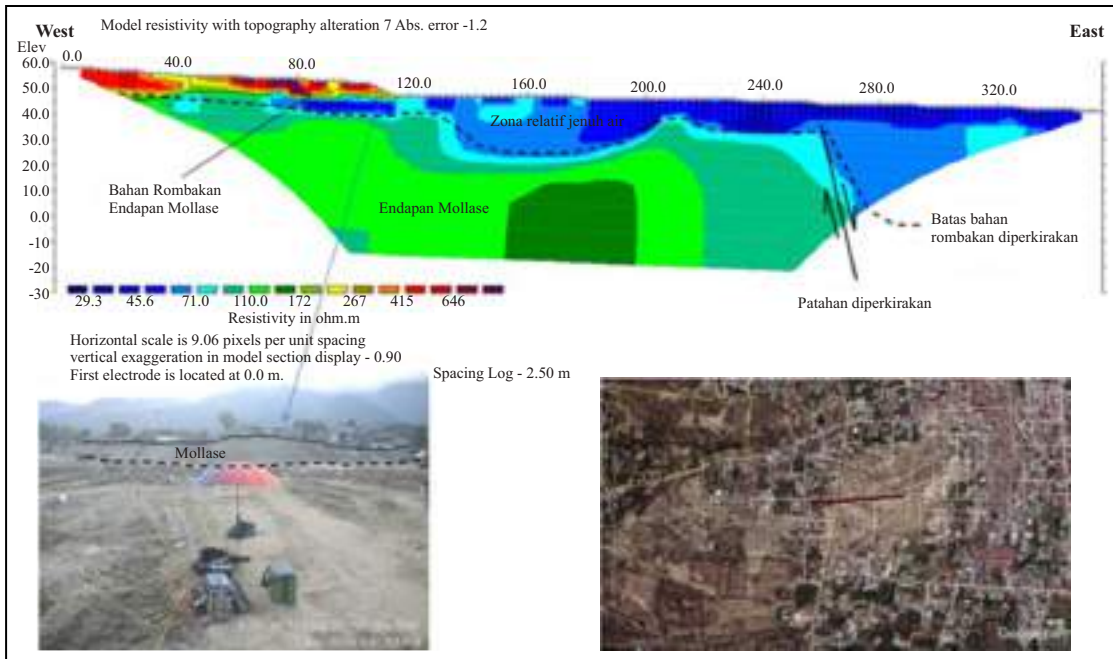
Figure 3.21. Interpretation of negative flower structure (red line dots) as a sign of strike slip fault based on electricity data from Taufiq et al. (2019).
