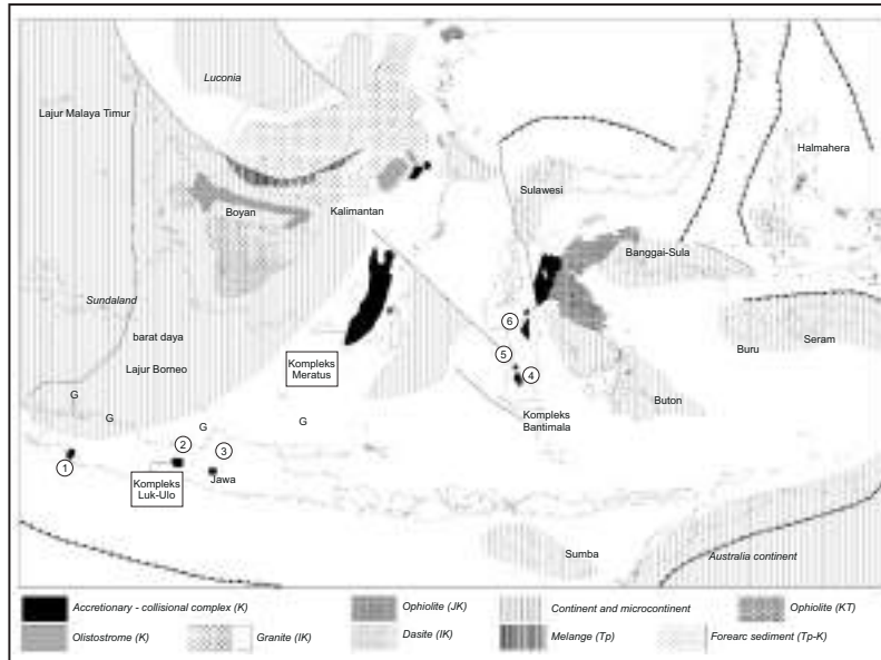
Figure 2.2. Major components of the Cretaceous accretionary-collision complex are distributed between a continent (Sundaland) and a microcontinent (Paternoster, Buton, etc.). Late Cretaceous accretionary-collision complexes are distributed in the following areas, i.e. 1. Cileutuh, 2. Karangsambung, 3. Jiwo Hills, 4. Bantimala, 5. Barru, 6. Pompango, 8. Meratus, and 9. Pulau Laut. Abbreviations of ages are as follows: JK: Jurassic to Cretaceous, K: Cretaceous, IK: Early Cretaceous, mK: Middle Cretaceous, uK: Late Cretaceous, Tp: Palaeogene, KT: Cretaceous to Tertiary (redrawn from Wakita, 2000).
