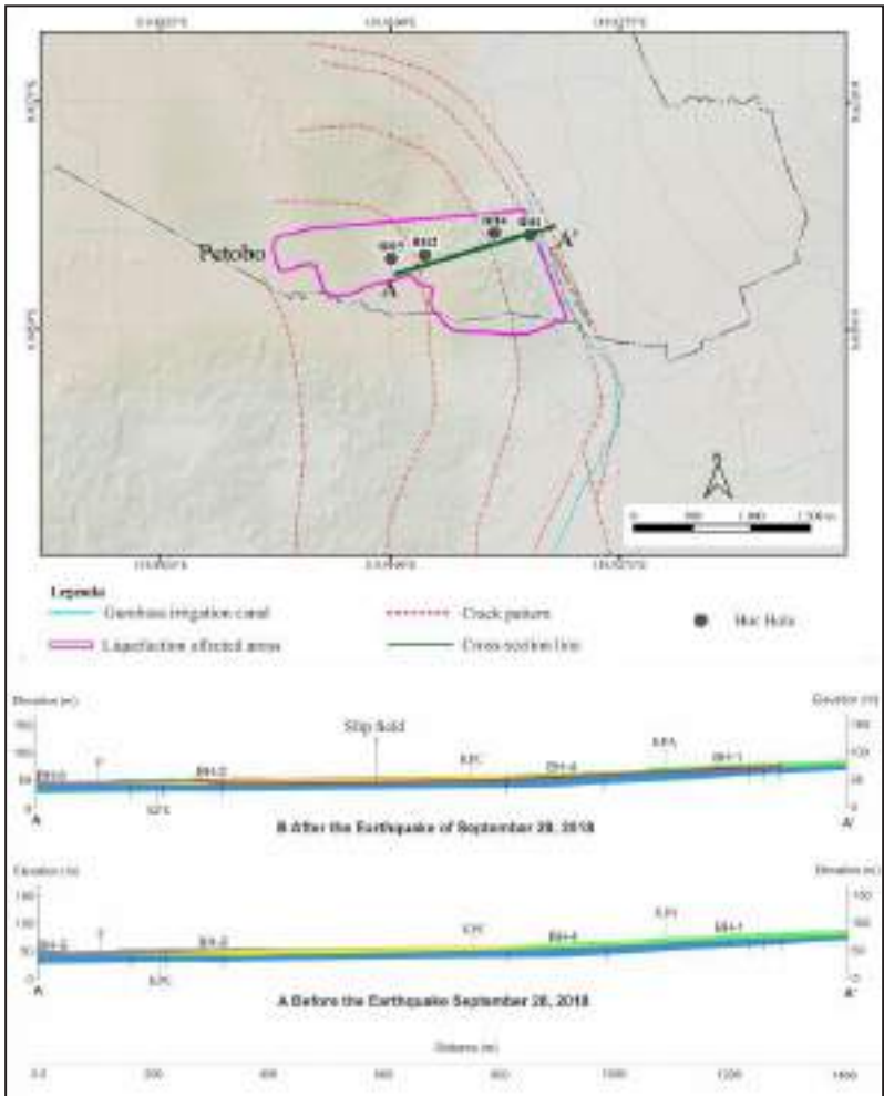
Figure 4.3.28. Reconstruction of the slip surface (red line) of the Petobo, and the results of calculations of safety factors against liquefaction.
