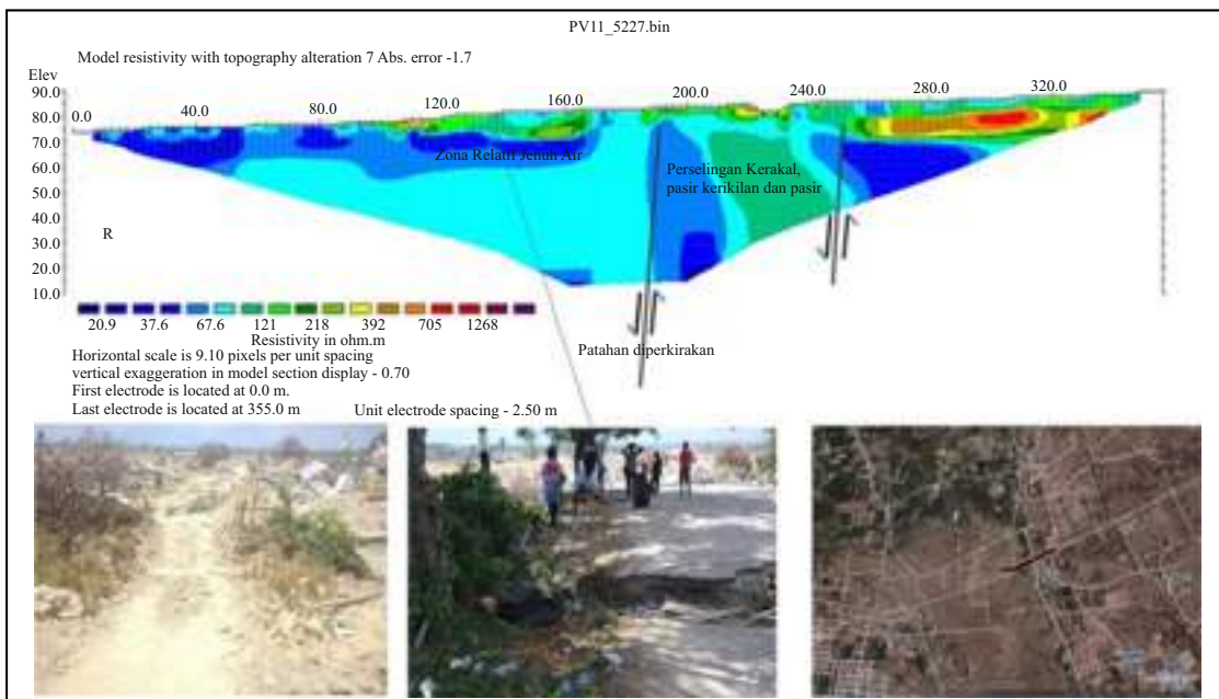
Figure 3.22. Interpretation of negative flower structure (dots red line) as a sign of strike slip fault based on electricity data from Buana et al. (2019).
