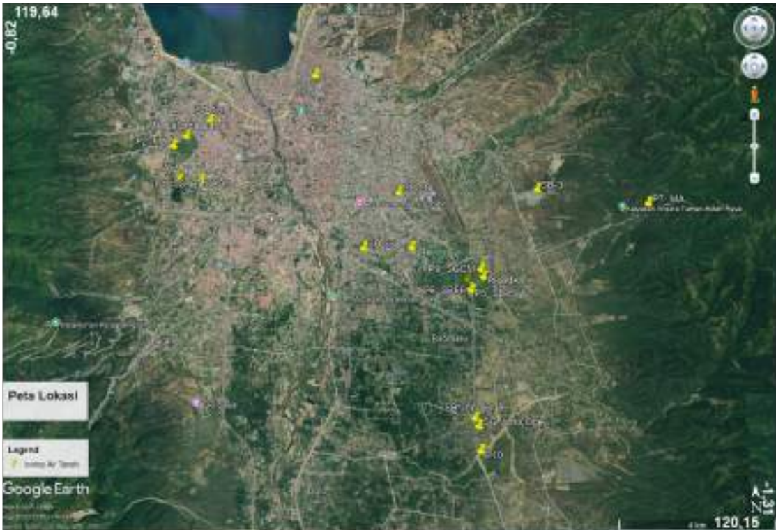
Figure 4.2.2. Distribution of groundwater isotope data collection points.
