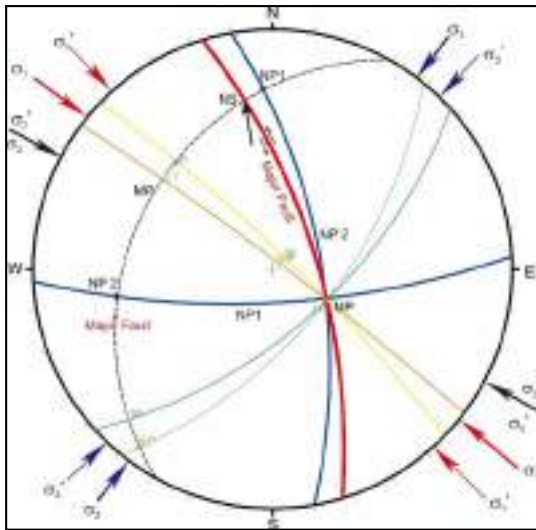
Figure 3.24. Stereonet analysis results of the Palu-Koro Fault Zone Movement Mechanism (Based on Earthquake Parameter Data from USGS).
